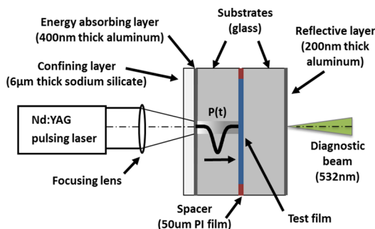
Figure 2. Schematic depiction of laser-induced shockwave experimental test setup and specimen structure.
